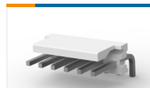
TE Part # 640389-6 06P MTA156 HDR ASSY SQ R/A F/L
